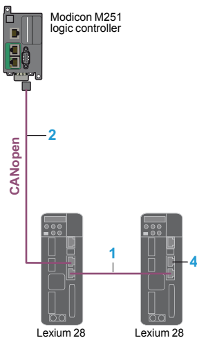
Example of architectures with control by Modicon M241/M251 logic controllers or LMC058 motion controller
